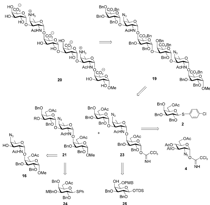
Scheme 5. Retrosynthetic analysis of hexasaccharide 19 .
